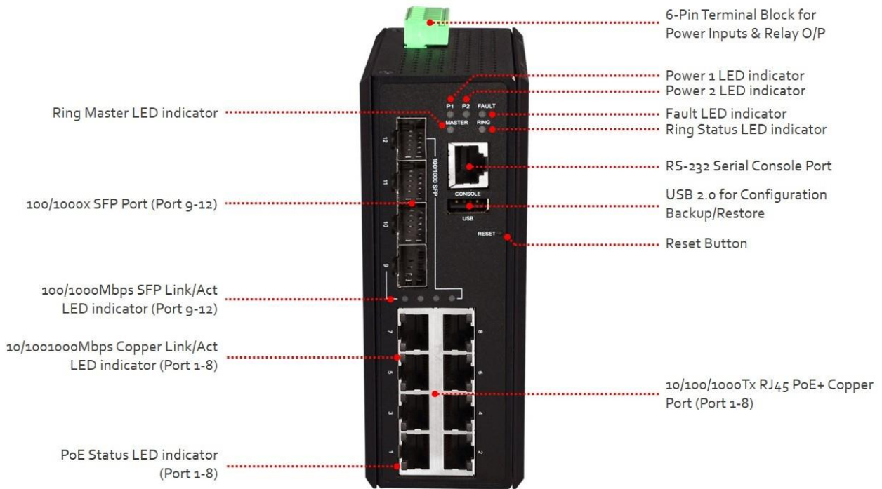
Figure 2.2: The Front Panel of WSI-1204-SFP-ATEX/Extd Series
