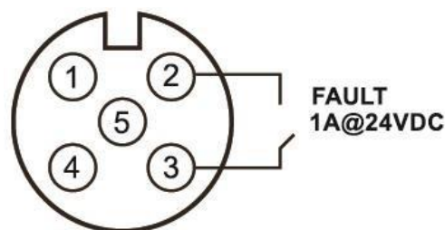
Figure 2.3: Wiring the relay contact for fault alarm
