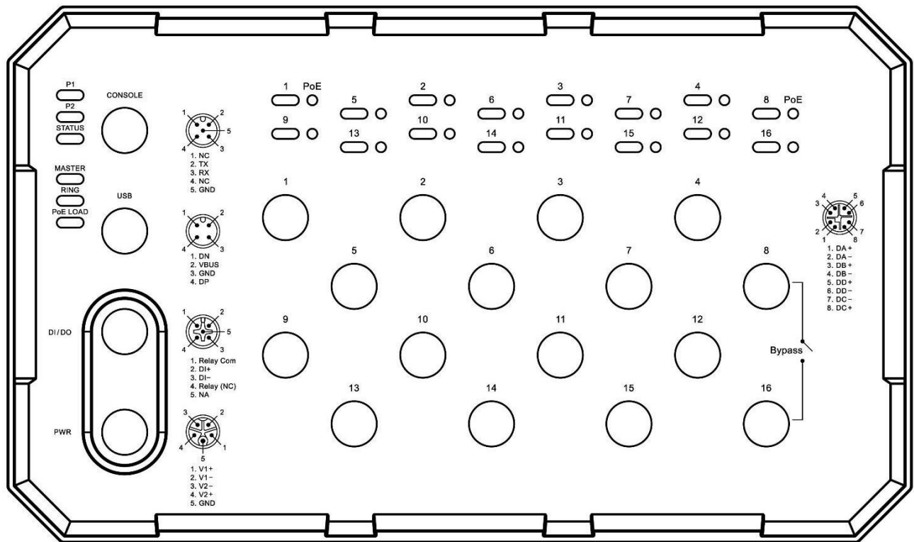
Figure 2.2: The Front Panel
