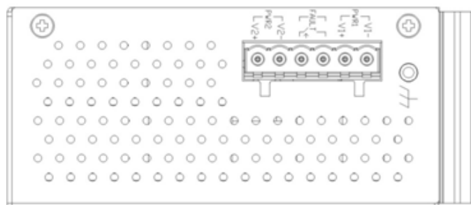
Figure 2.3: Top Panel View of WSI-0802-SFP(-24) Series
