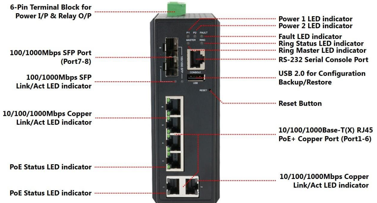
Figure 2.2: The Front Panel of WSI-0802-SFP(-24) Series
