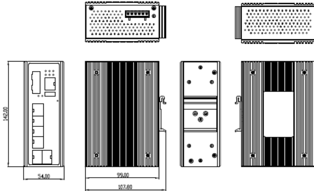
Figure 2.1: WSI-0802-SFP(-24) Series Physical Dimensions
